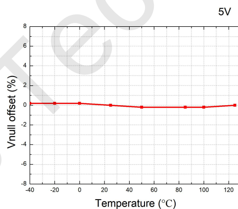
Typical Temperature (T A ) VS V NULL Offset
